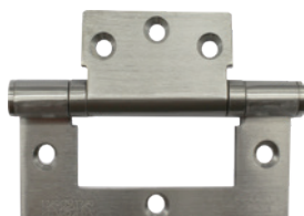
Flush Hinge SH100SSBL Hinge Flush 100x41x2.5mm B/Bearing SS Pair Blister
